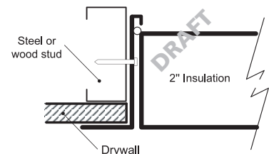
[ 1 HOUR CEILING APPLICATION ]
