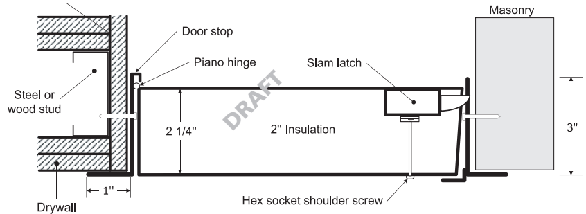
[ 3 HOUR CEILING APPLICATION ]
